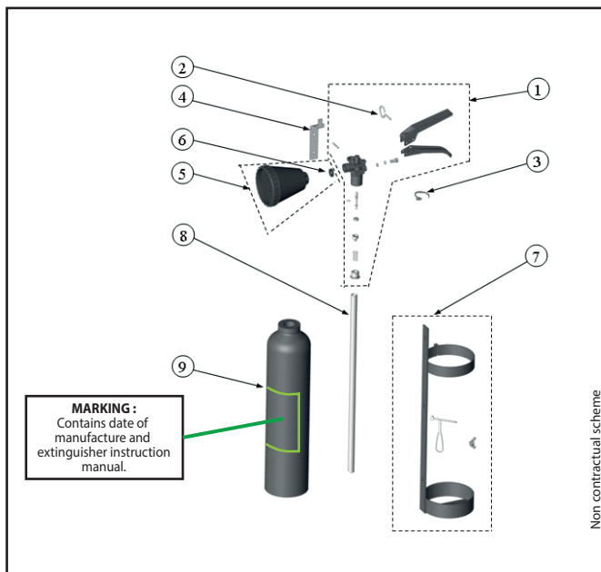
EXTINGUISHER SCHEMA
